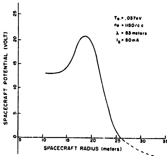
Figure 8. - Nonmonotonic behavior of spacecraft potential as a function of spacecraft radius, for a given electron beam current.
