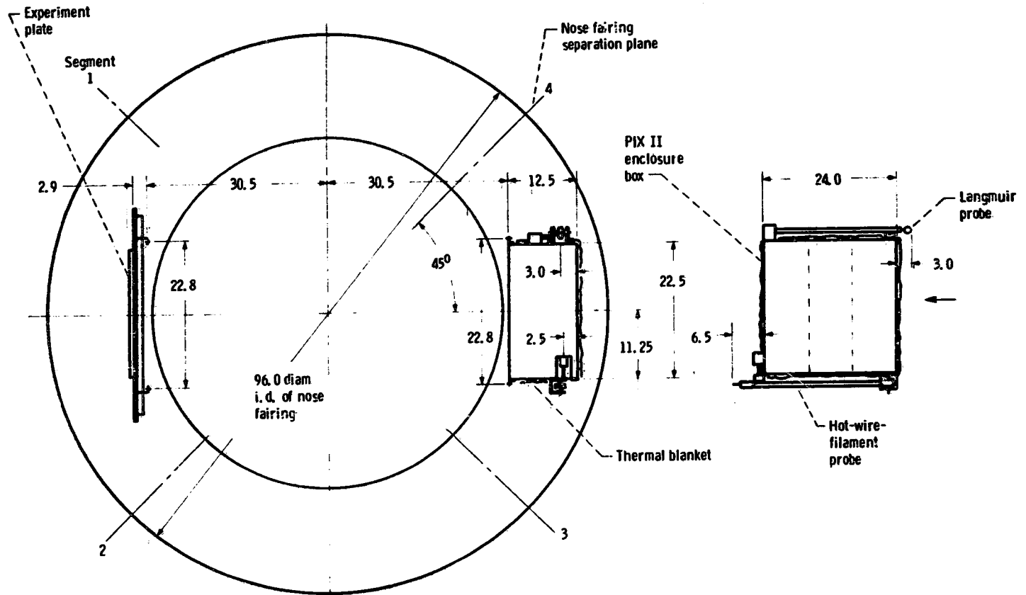
Figure 1. - PIX II/Delta. (Dimensions are in inches.)
