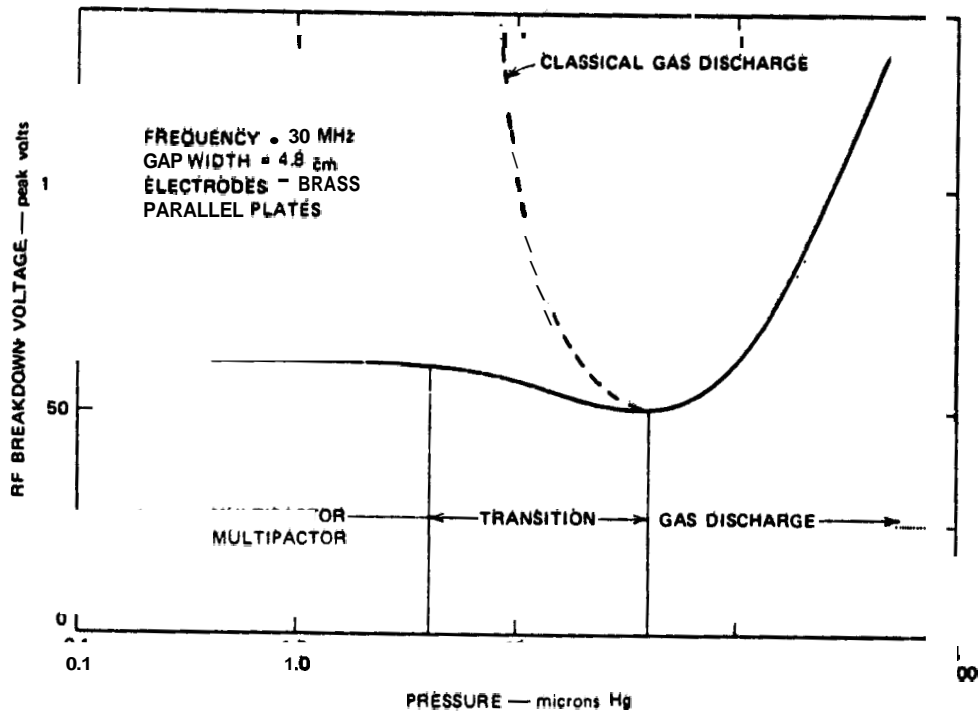
Figure 1. Variation of R F Breakdown voltage With Pressure
