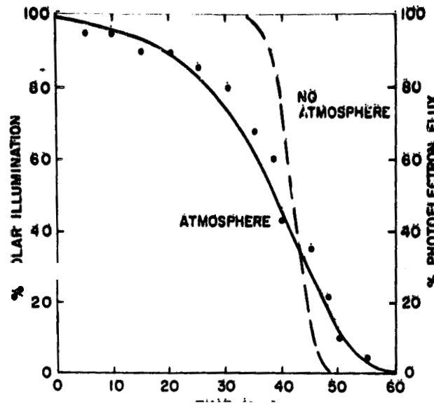
Figure 7. INJUN V Measurements of the Photo-electron Flux as a Function of Time in the Penumbra Region (Dots). Also shown are two theoretical curves of the solar illumination for the case of no atmosphere (dashed line) and with an atmosphere (solid line)
