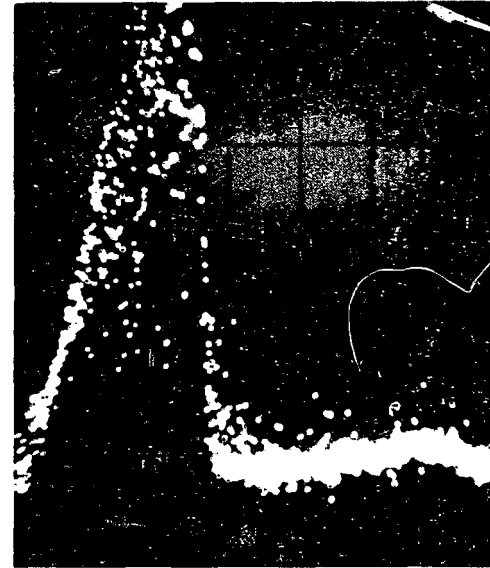
Figure 2. Micro-Discharge Current Pulse Measured Under Same Conditions as Figure 1, Except that the Spot Beam has been Moved to a Different Area on the Same Specimen
