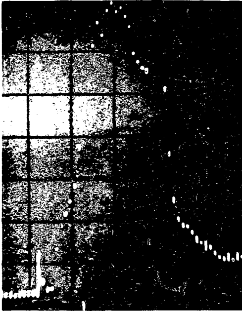
Figure 1. Micro-Discharge Current Pulse as Measured With a Sampling Oscilloscope. The upward direction corresponds to current flowing downward from the pedestal on which rests the Teflon specimen, measuring 10 \times 10 \times 0.5 mm. The 18 kV electron beam is highly focussed and only a small area of the Teflon is exposed to it. Horizontal scale 1 ns/div and vertical scale 100 mA/7 div
