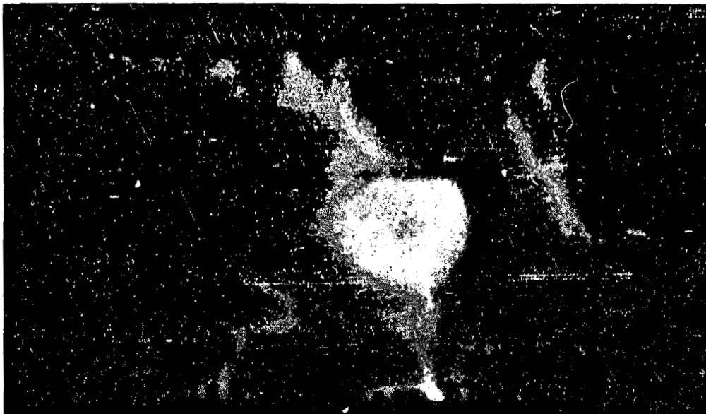
Figure 3. Macro-Discharge on Surface of Mylar Specimen 26 \times 48 \times 0.12 mm. The primary arc discharge goes from the central bright spot (due to filament illumination) to the lower edge of the specimen. The other bright areas are luminescence. The beam accelerating voltage is 20 kV
